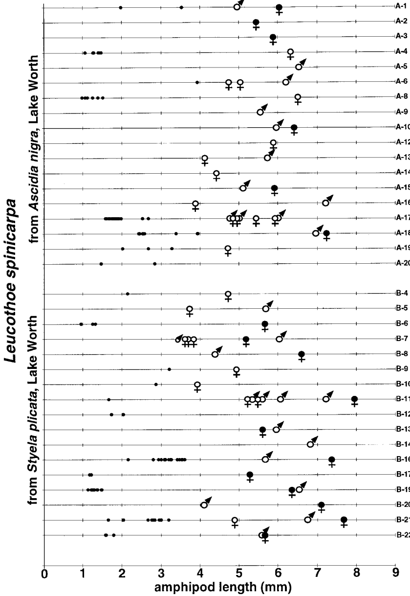
FIG. 4 Sizes of Leucothoe spincarpa in solitary and stolonal ascidians; numbers A-1 to F-24 represent all solitary ascidians containing amphipods; symbols represent amphipods within ascidians: dots—immatures; male symbol—mature males, open female symbol—mature females with empty brood pouch, filled female symbol—mature ovigerous females; open squares—immatures from stolonal ascidians; squares with female symbol—immature females; all amphipods from zooids of stolonal ascidians collected at one sampling site and date were pooled.
